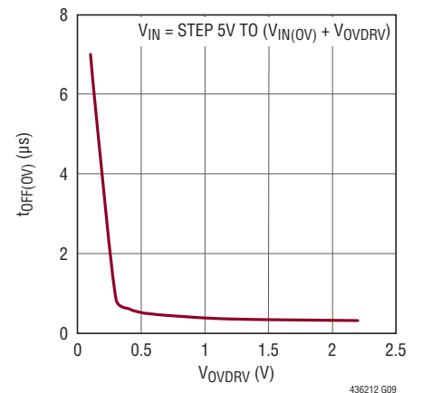
Overvoltage Turn-Off Delay vs Overdrive ( V_{OVDIV} )
