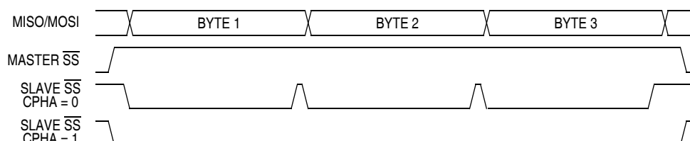
Figure 15-6. CPHA/\overline{SS} Timing
