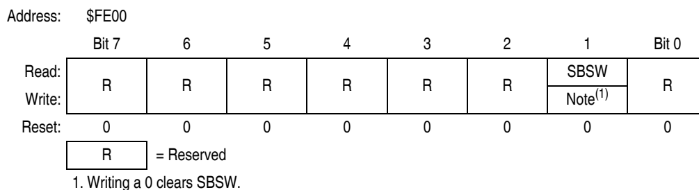
Figure 14-20. Break Status Register (SBSR)
