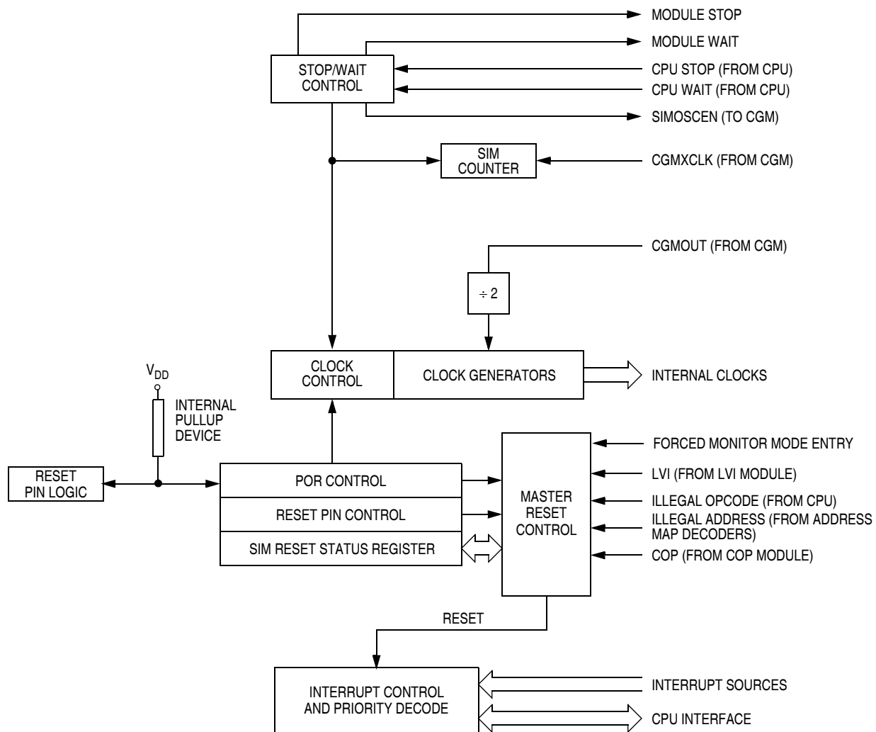
Figure 14-1. SIM Block Diagram
