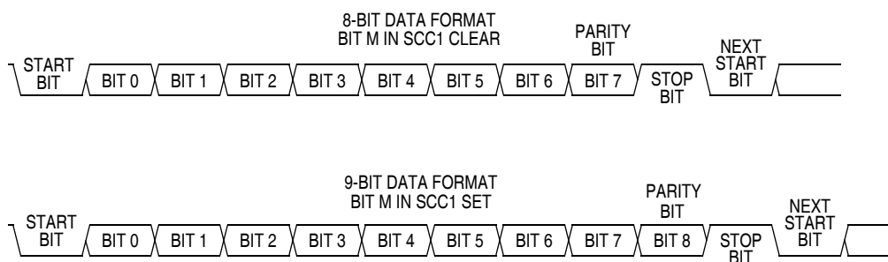
Figure 13-2. SCI Data Formats
