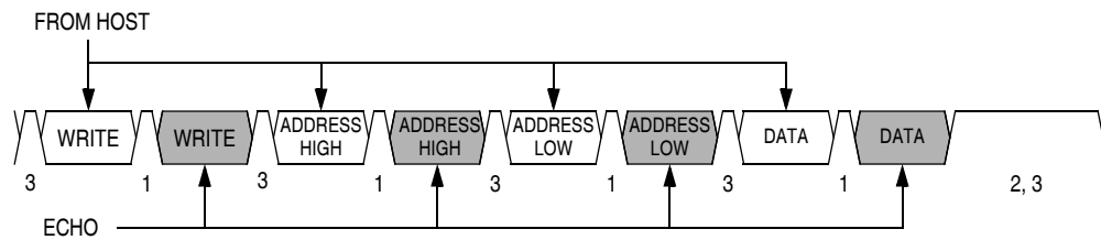
Figure 18-14. Read Transaction
