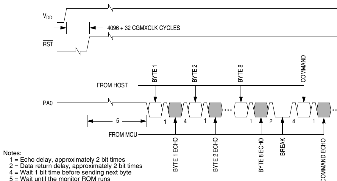
Figure 18-17. Monitor Mode Entry Timing
