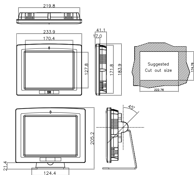
AFL-08AH-N270
