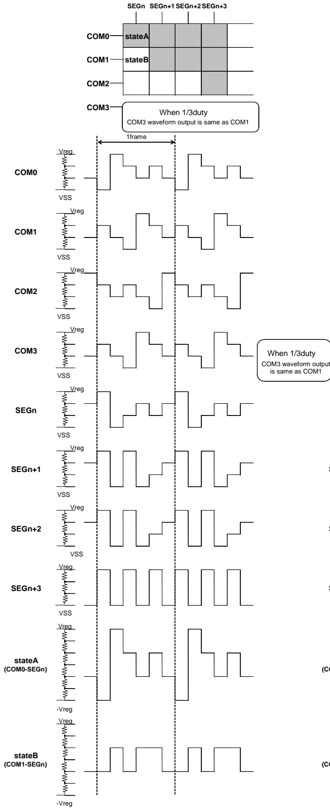
Figure 11. LCD Drive Waveform during Line inversion
