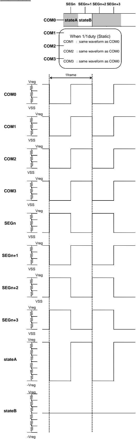
Figure 13.LCD Drive Waveform during Line inversion Figure 14. LCD Drive Waveform during Frame inversion
