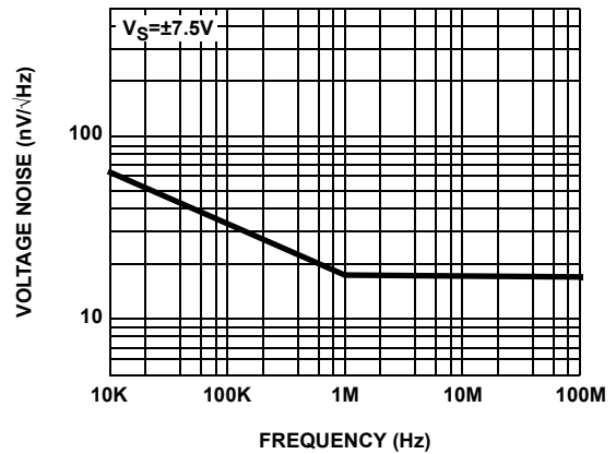
FIGURE 14. INPUT NOISE SPECTRAL DENSITY vs FREQUENCY ( V_{COM} )
