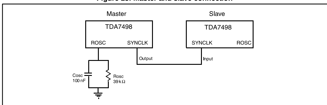
Figure 23: Master and slave connection
