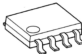
SOP8-P-225-1.27
