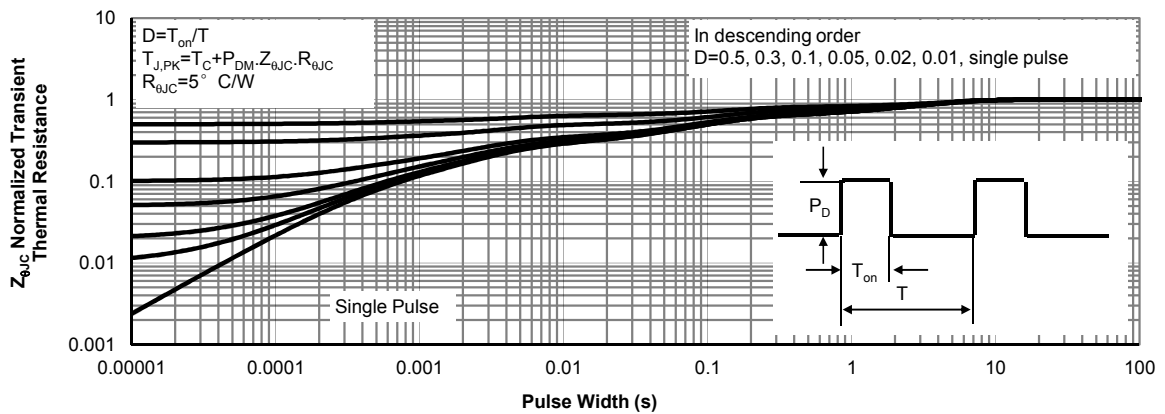
Figure 11: Normalized Maximum Transient Thermal Impedance for AOWF4N60 (Note F)
