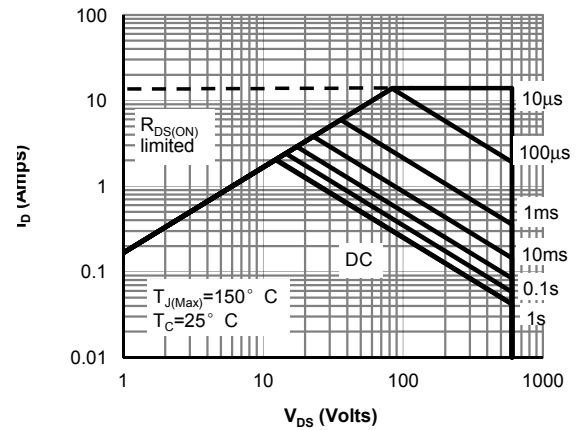
Figure 10: Maximum Forward Biased Safe Operating Area for AOWF4N60 (Note F)
