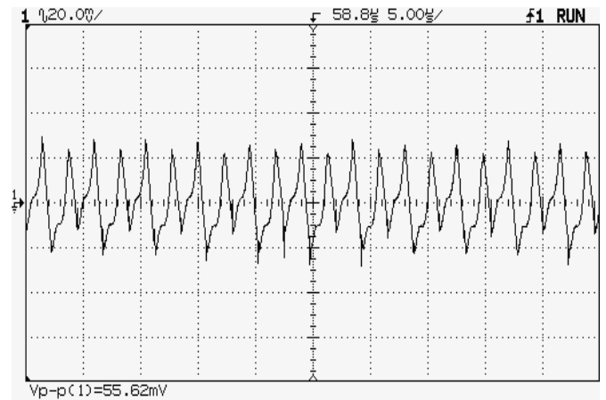
Output Ripple and Noise (Vin=48V, Io=40A, 100Mz BW)
