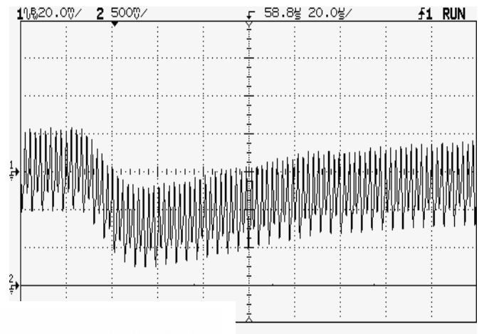
Output Voltage Response to Step Load (20A → 30A load step, di/dt = 1A/us, Tamb=25C, Vin=48V)
