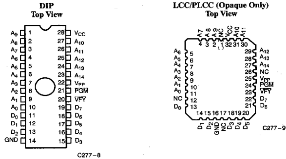
Figure 1. Programming Pinouts
