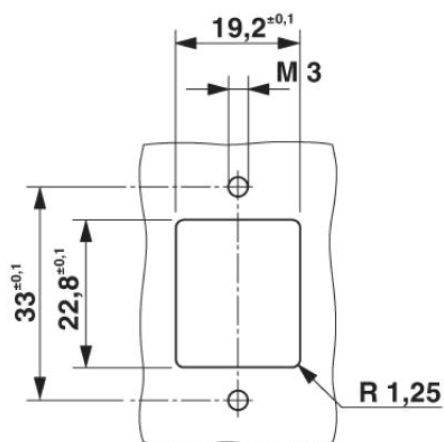
Panel cutout
