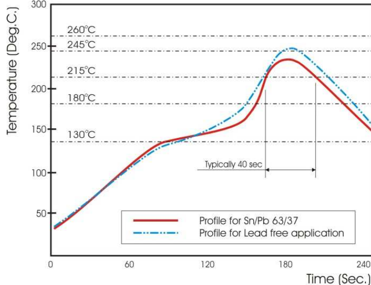
Fig 3. Infrared soldering profile for Chip Resistors WW25
