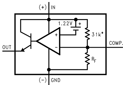
Figure 1. LM3460 Functional Diagram
