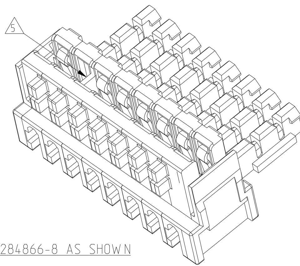
- - - SEE TABLE PH. BRONZE, TIN PLATED IDC RECEPTACLE CONTACT PBT GLASS FIBER FILLED FEMALE HOUSING Q.TY MATERIAL DESCRIPTION 1 REVISIONE DELL'ASSEMBLATO (REVISION OF EACH ASSY NO) G.14) PER ASSEMBLATO (QTY REQ'D PER ASSY) ELenco DEI COMPONENTI (PARTS LIST)
