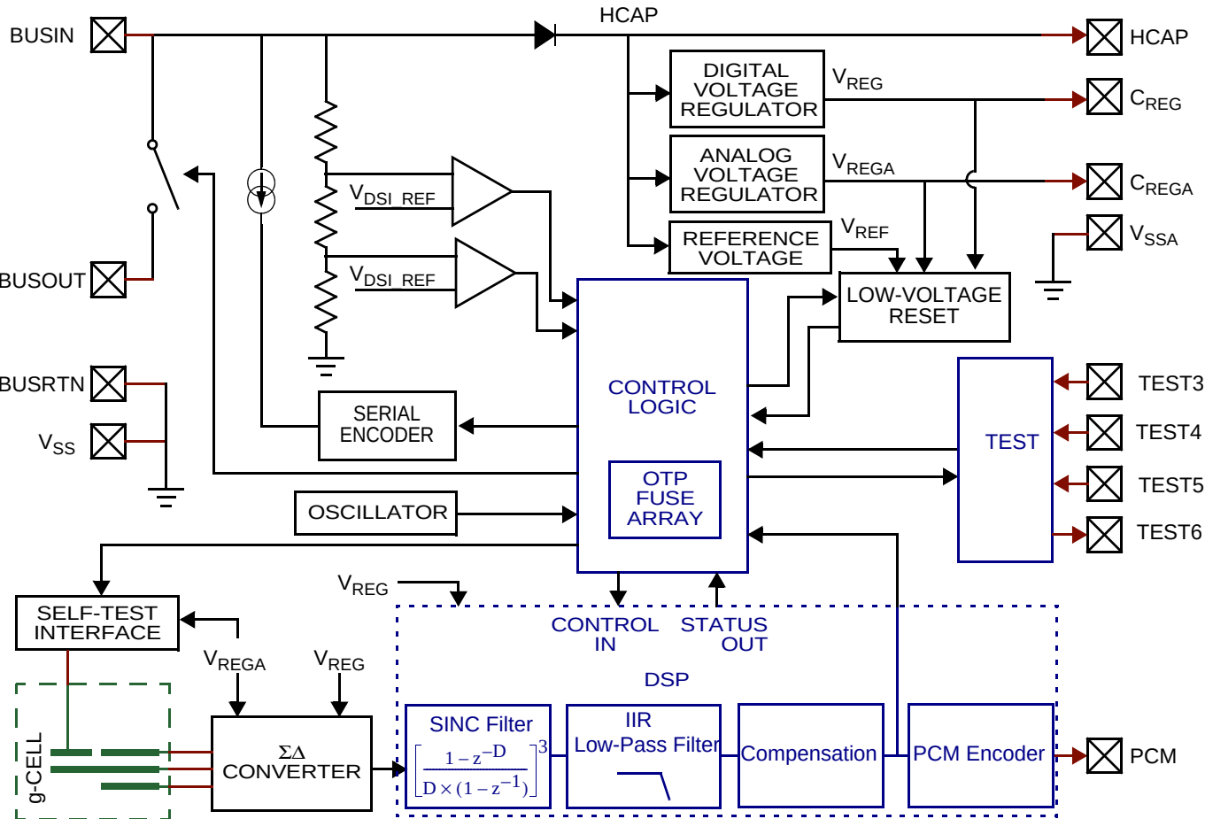
Figure 3. Block Diagram9
