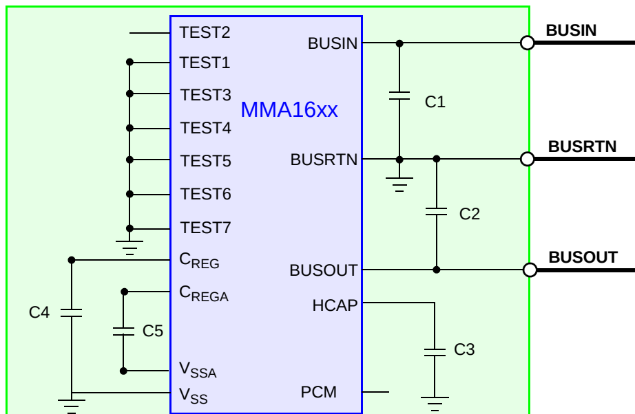
Figure 1. Application Diagram
