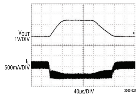
V OUT Short to V IN (Forced Continuous Mode)
