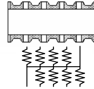
745C102 8 Resistors 10 Terminations
