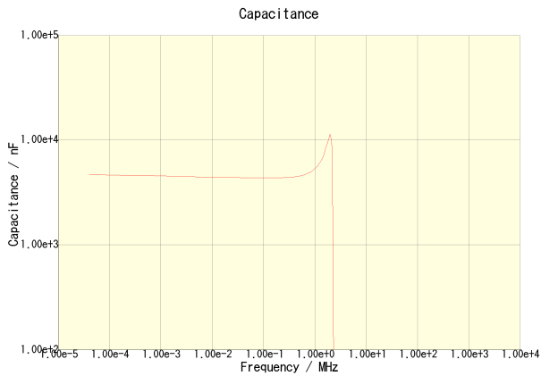
C2012X5R0J475K125AA
