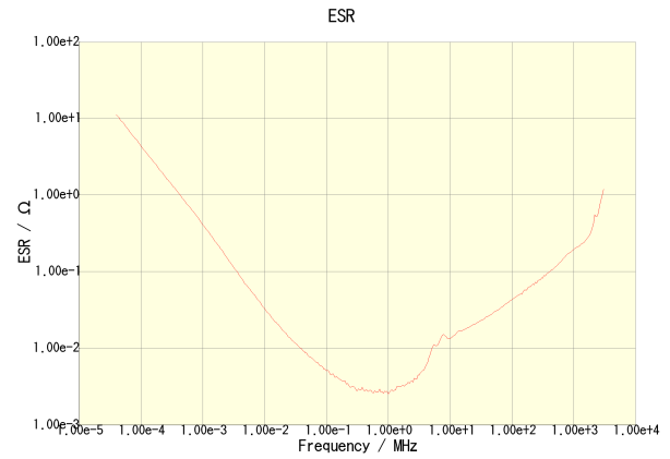
C2012X5R0J475K125AA
