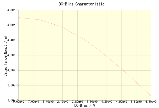
C2012X5R0J475K125AA
