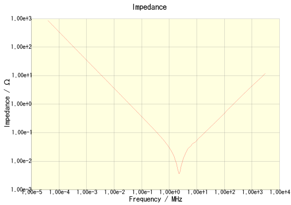
C2012X5R0J475K125AA
