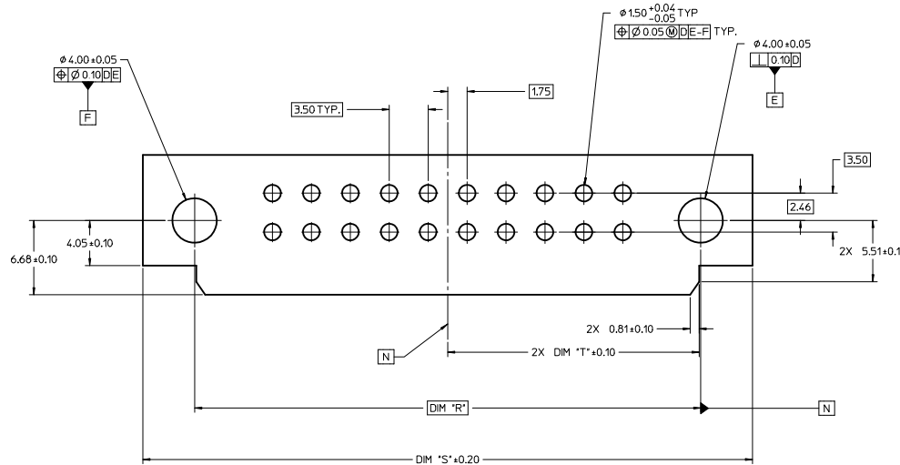
PCB LAYOUT FOR EON TOWARD HARNESS CONNECTOR
