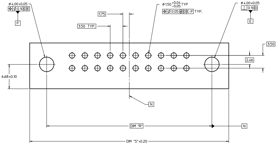
PCB LAYOUT FOR SOLDERTAIL TOWARD HARNESS CONNECTOR
