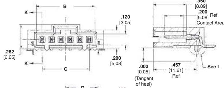
Section K-K
