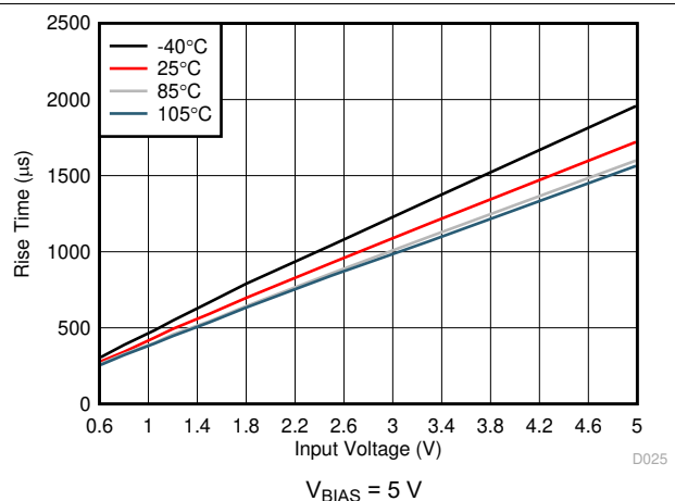
Figure 6-30. Rise Time vs Input Voltage
