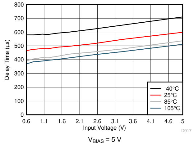
Figure 6-20. Delay Time vs Input Voltage
