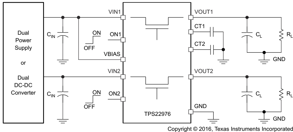
Figure 9-5. Typical Application Circuit
