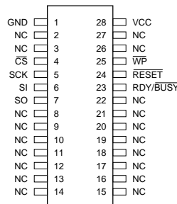
PLCC
