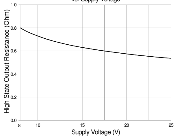
Fig. 22 High State Output Resistance vs. Supply Voltage
