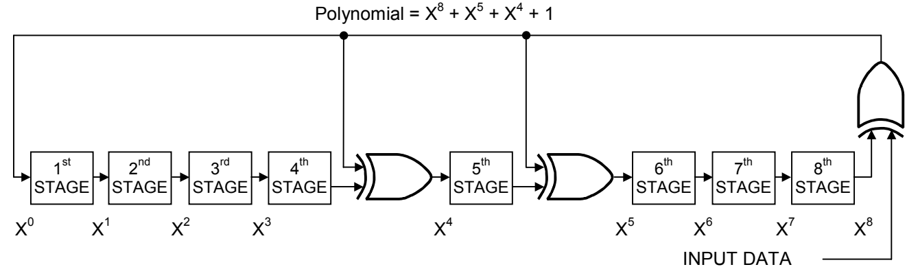
Figure 6. 1-Wire CRC Generator
