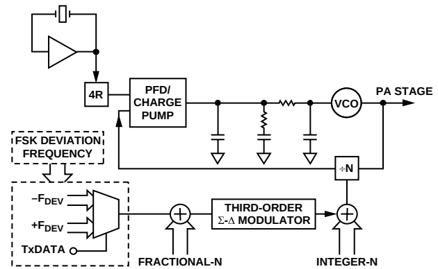
Figure 28. FSK Implementation
