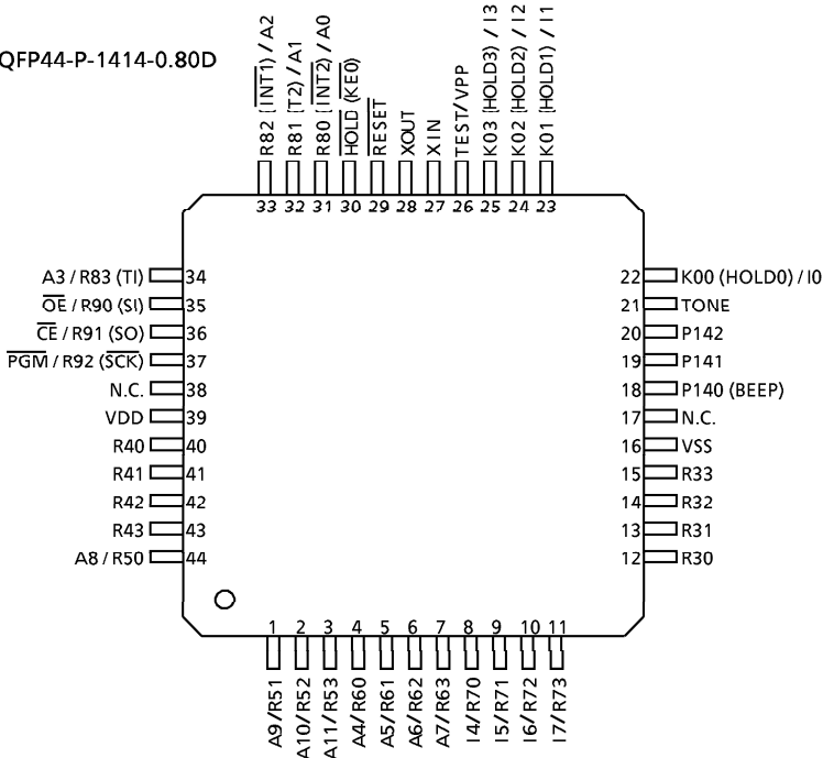
QFP44-P-1414-0.80D
