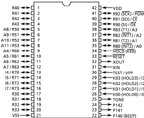
SDIP42-P-600-1.78
