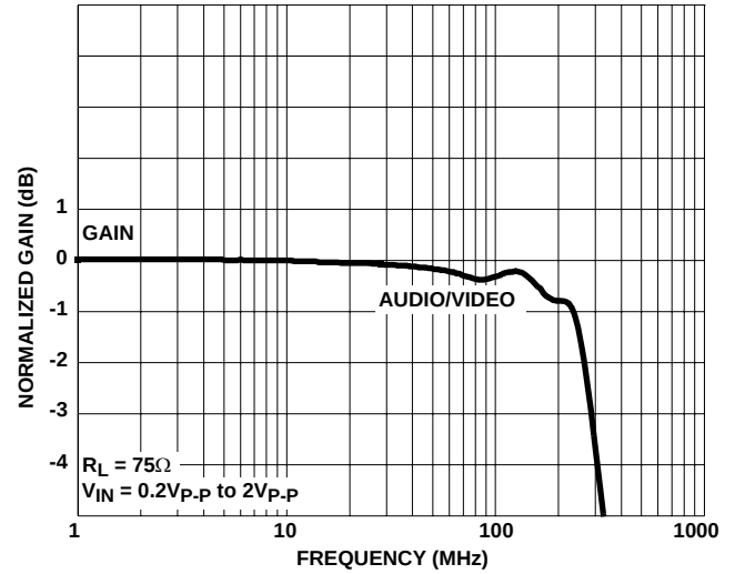
FIGURE 14. FREQUENCY RESPONSE
