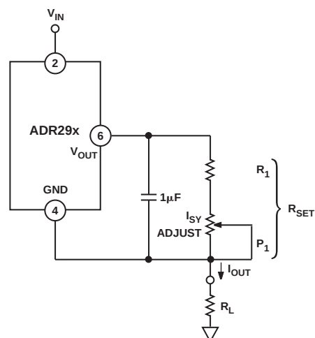
Figure 33. A Precision Current Source
