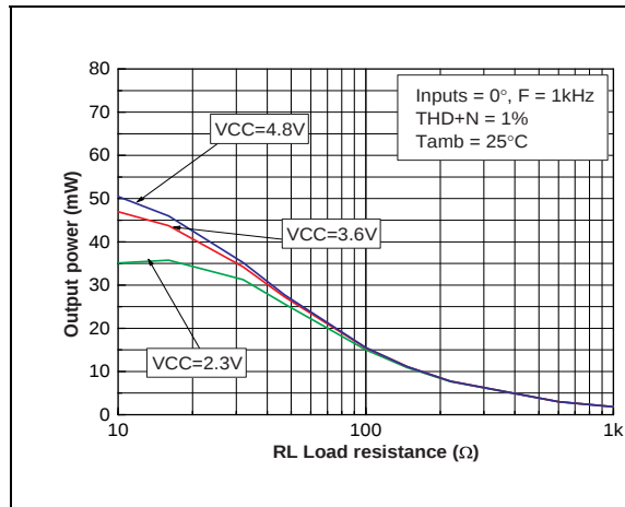
Figure 6. Maximum output power vs. load
