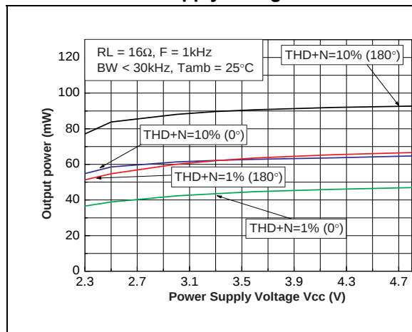
Figure 8. Maximum output power vs. power supply voltage
