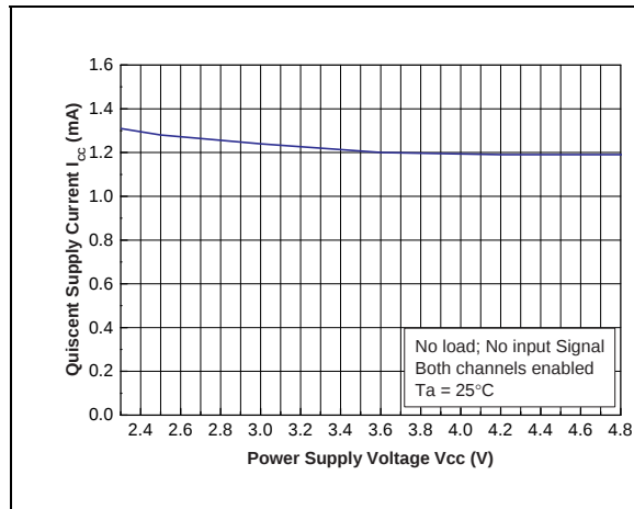
Figure 4. Current consumption vs. power supply voltage
