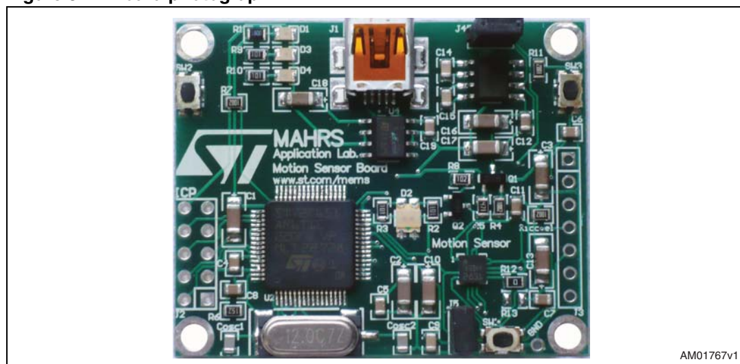
Figure 3. Board photograph
