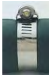
Hose installed with lined clamp
