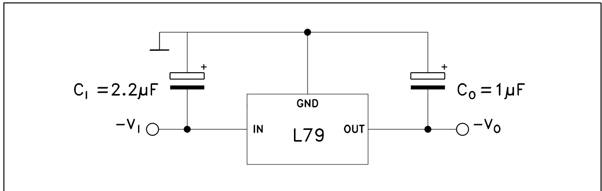
Figure 3. Test circuit
