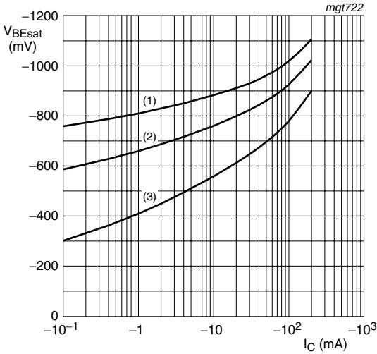
Fig 10. BCV62C: Base-emitter voltage as a function of collector current; typical values
