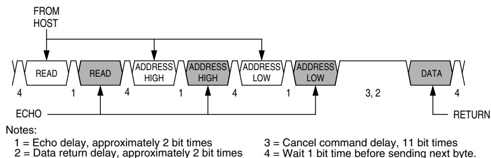
Figure 18-15. Read Transaction
