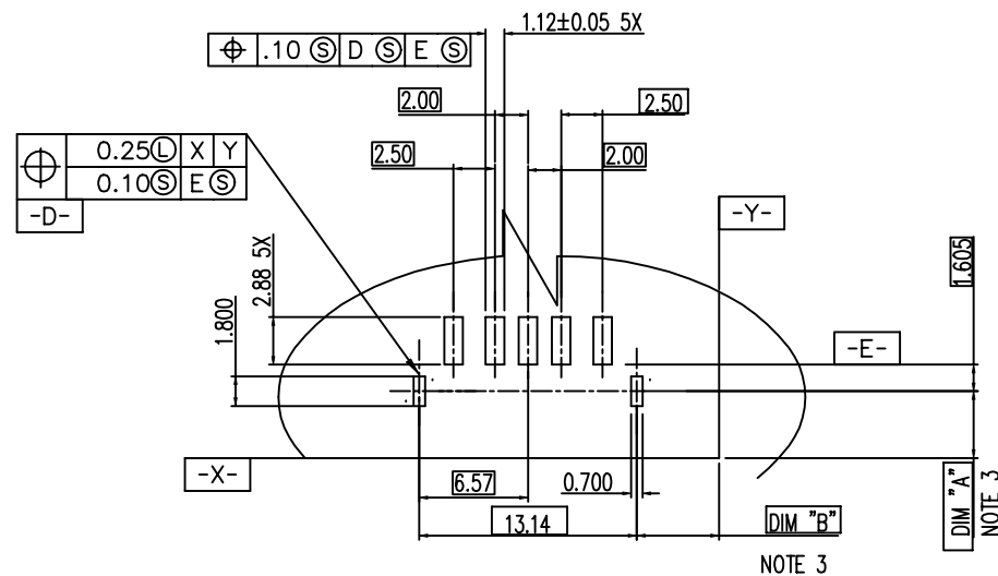
P.C. BOARD LAYOUT
