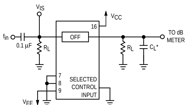
Figure 6. Off-Channel Feedthrough Isolation, Test Set-Up
