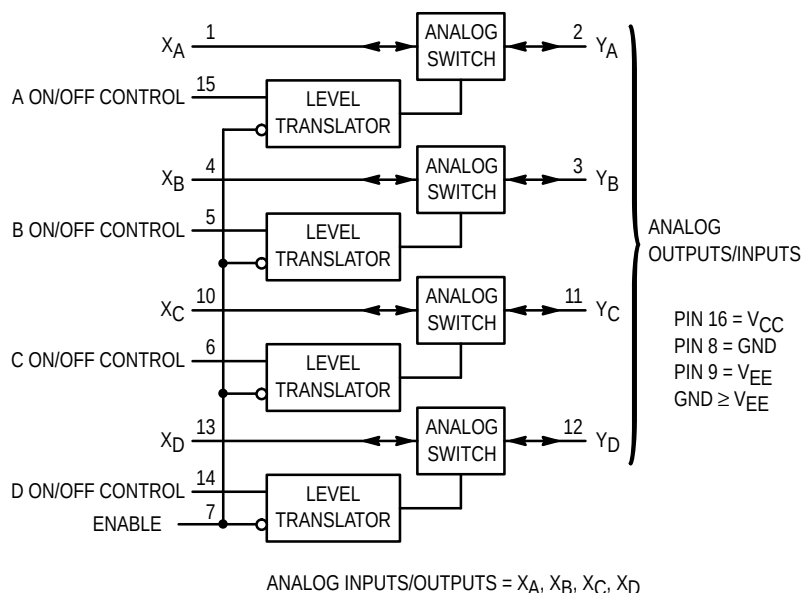
LOGIC DIAGRAM
