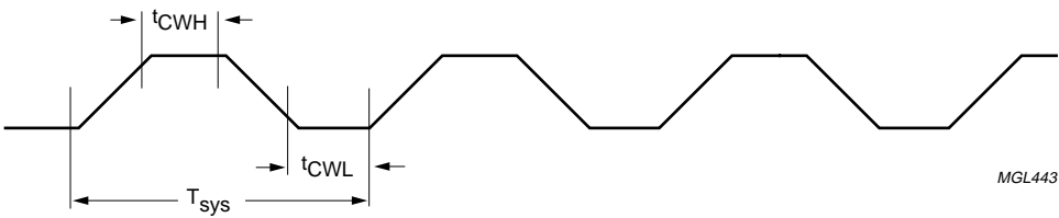
Fig.8 System clock timing.
