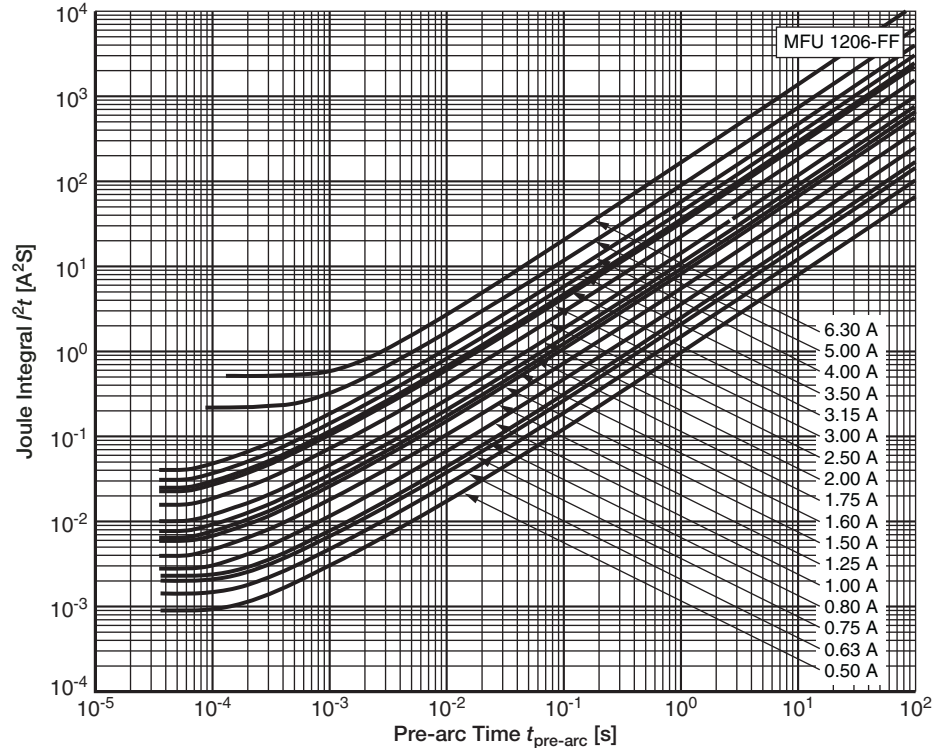
Typical I^2t vs. t_{\text{pre-arc}} characteristic of MFU 1206 (1)
