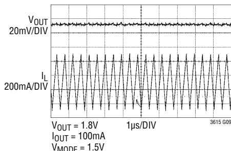
Forced Continuous Mode Operation (FCM)
