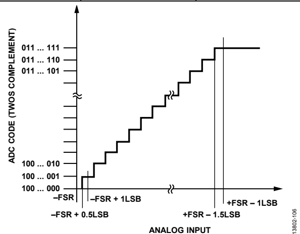
Figure 106. Transfer Function
