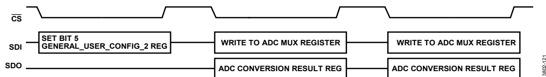
Figure 121. Configuring the AD7771 to Operate the SPI to Read from the SAR ADC
