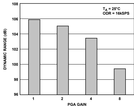
Figure 52. Dynamic Range vs. PGA Gain at 16 kSPS, High Resolution Mode
