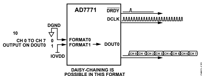
Figure 132. FORMATx Pin Configuration—FORMAT0 = 0, FORMAT1 = 1
