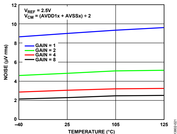
Figure 21. Noise vs. Temperature at 16 kSPS, High Resolution Mode, Sinc3 Filter Enabled
