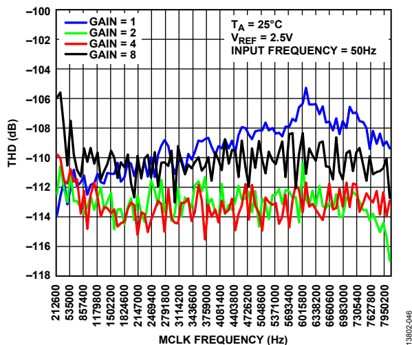
Figure 46. THD vs. Master Clock Frequency, High Resolution Mode
