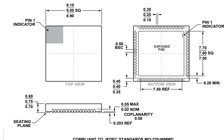
Figure 139. 64-Lead Lead Frame Chip Scale Package [LFCSP] 9 mm × 9 mm Body and 0.75 mm Package Height (CP-64-15)
