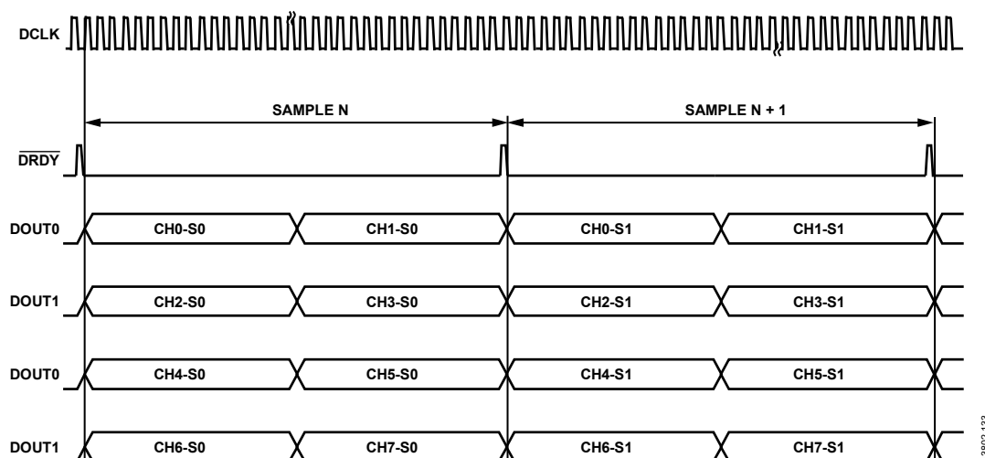
Figure 133. FORMAT0 = 0 , FORMAT1 = 0 —Each DOUTx Outputs Two ADC Conversions (S0 Means Sample 0 and S1 Means Sample 1)
