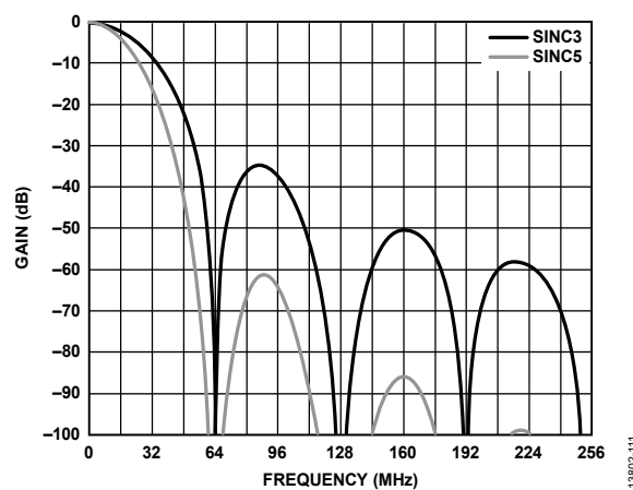
Figure 111. Sinc3/Sinc5 Frequency Response in High Resolution Mode
