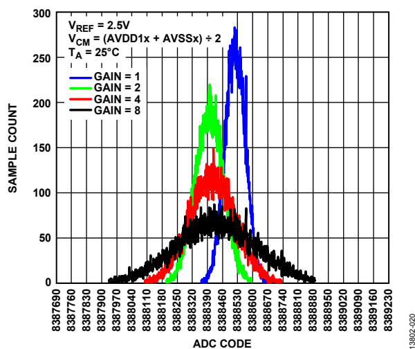
Figure 20. Noise Histogram at 64 kSPS, High Resolution Mode, Sinc5 Filter Enabled
