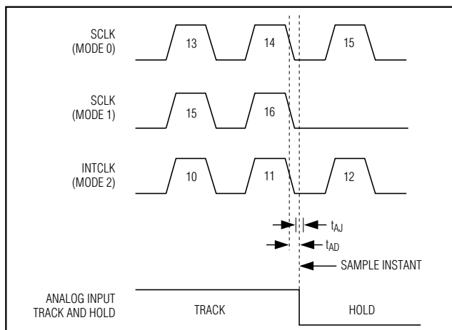
Figure 21. Aperture Diagram
