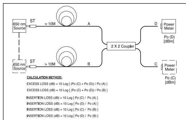
FIGURE 2. Excess & insertion loss measurement - (post-fused)
