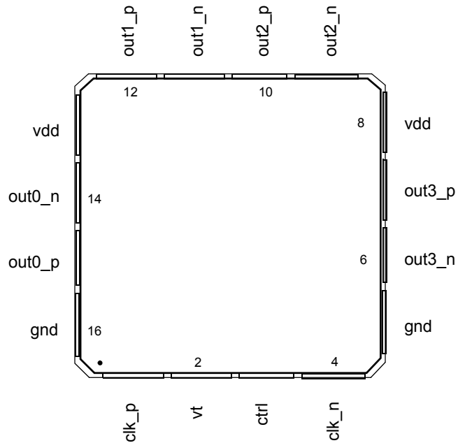
Figure 2 - Pin Connections
