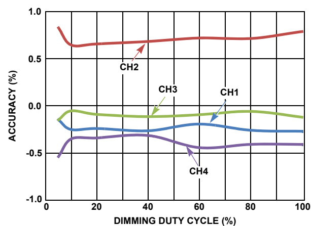
FIGURE 7. ACCURACY vs WPM DIMMING ( V_{IN} : 24V, V_{OUT} : 55V FOR 4P18S, I_{CH} : 100mA)
