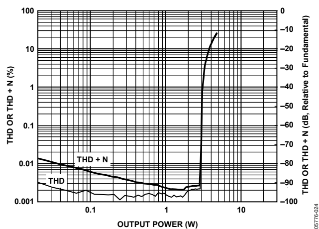
Figure 24. THD and THD + N vs. Output Power, 1 kHz Sine, 8 Ω Load, PVDD = 12 V
