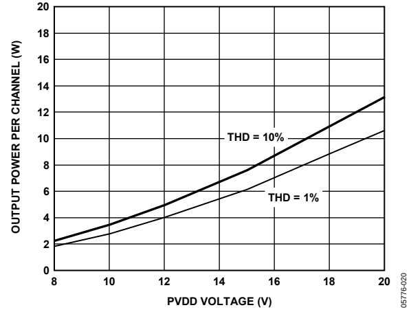
Figure 20. Maximum Output Power vs. PVDD, 6 Ω Load
