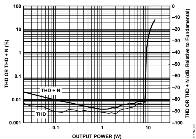
Figure 25. THD and THD + N vs. Output Power, 1 kHz Sine, 4 Ω Load, PVDD = 15 V
