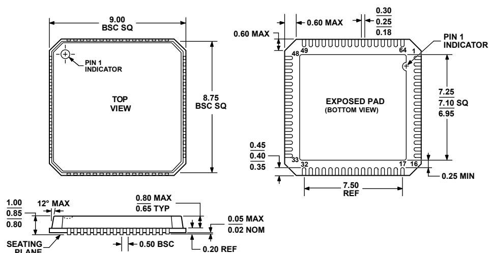
Figure 39. 64-Lead Lead Frame Chip Scale Package [LFCSP_VQ] 9 mm × 9 mm Body, Very Thin Quad (CP-64-3) Dimensions shown in millimeters
