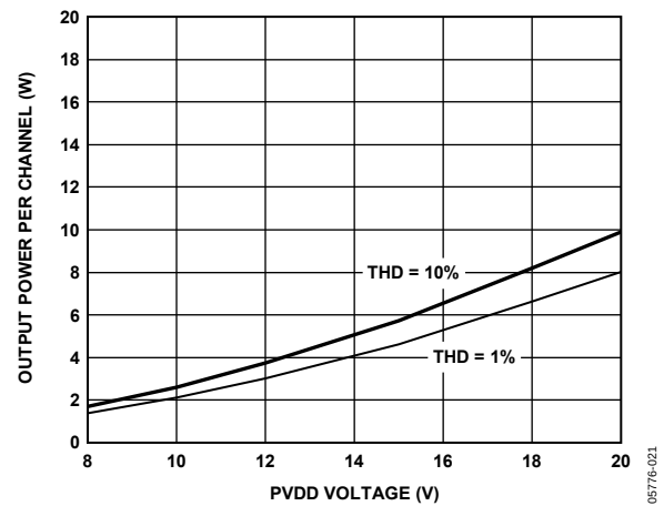
Figure 21. Maximum Output Power vs. PVDD, 8 Ω Load
