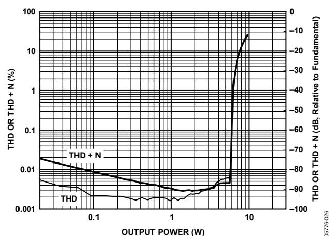
Figure 26. THD and THD + N vs. Output Power, 1 kHz Sine, 6 Ω Load, PVDD = 15 V
