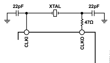
Figure 37. Crystal Connection
