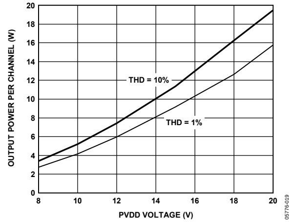
Figure 19. Maximum Output Power vs. PVDD, 4 Ω Load
