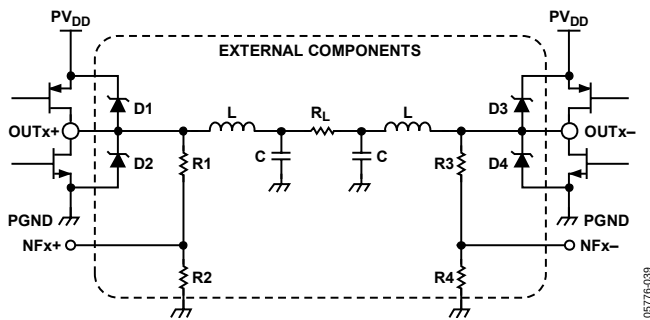
Figure 35. H-Bridge Configuration
