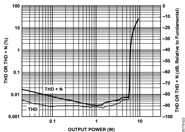
Figure 22. THD and THD + N vs. Output Power, 1 kHz Sine, 4 Ω Load, PVDD = 12 V
