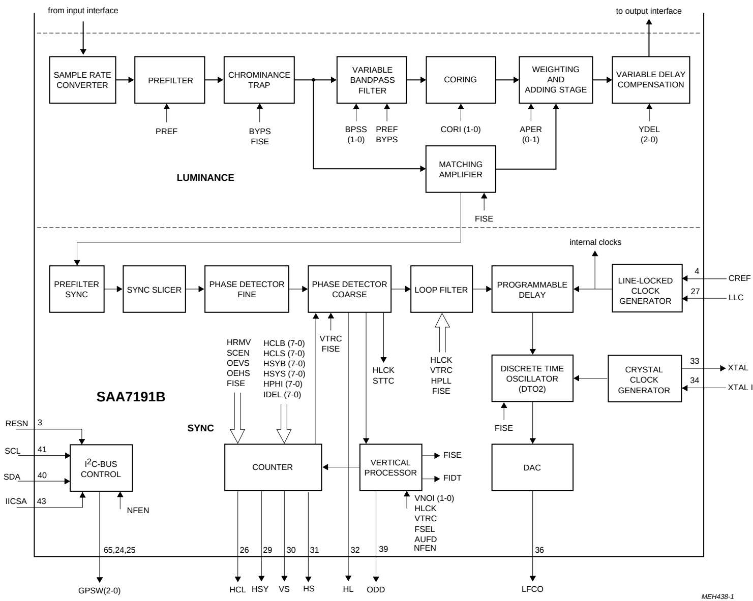
Fig.4 Detailed block diagram; continued from Fig.3.
