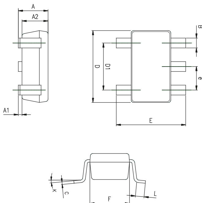
Figure 29. SOT23-5 package outline
