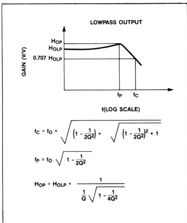
Figure 3. Lowpass Response
