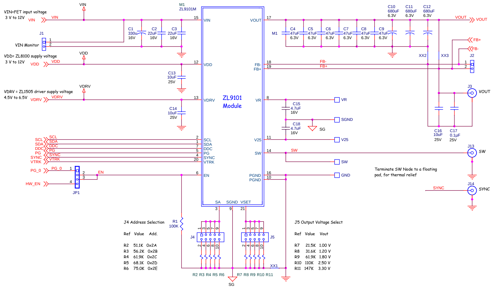
FIGURE 2. ZL9101EVAL1Z CIRCUIT SCHEMATIC
