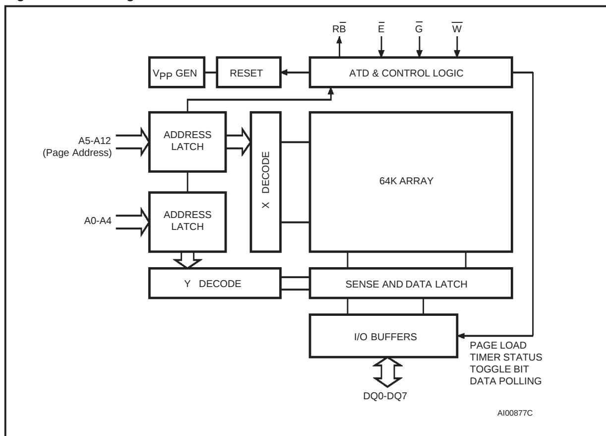
Figure 3. Block Diagram
